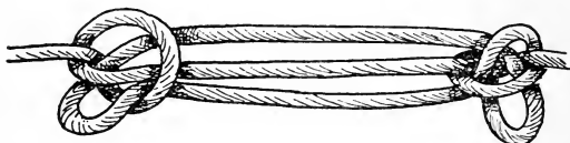
FIG. 78.—Sheepshank.
